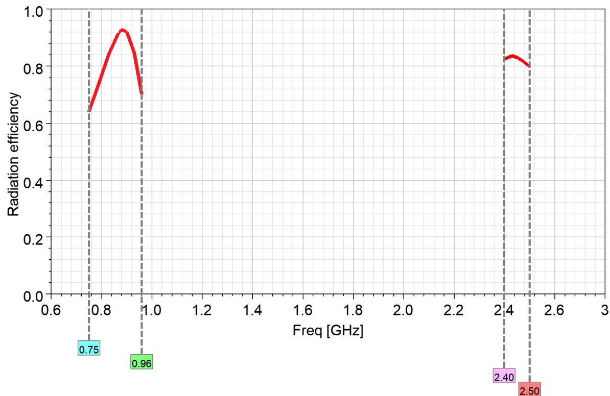
Radiation efficiency
