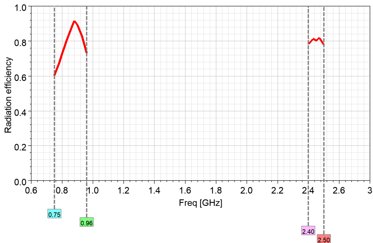
Radiation efficiency
