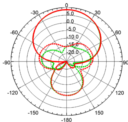
960 MHz
