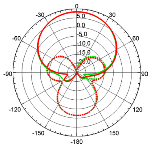
915 MHz
