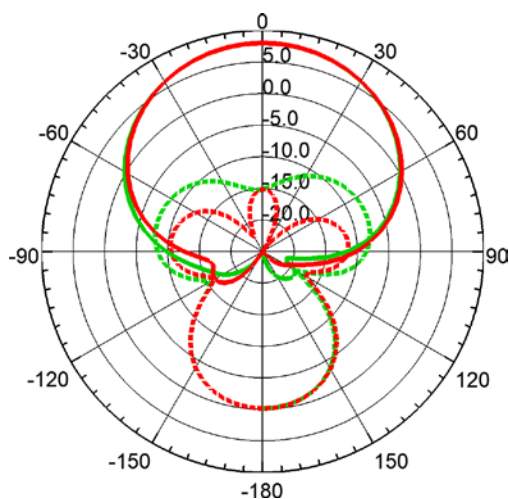
868 MHz
