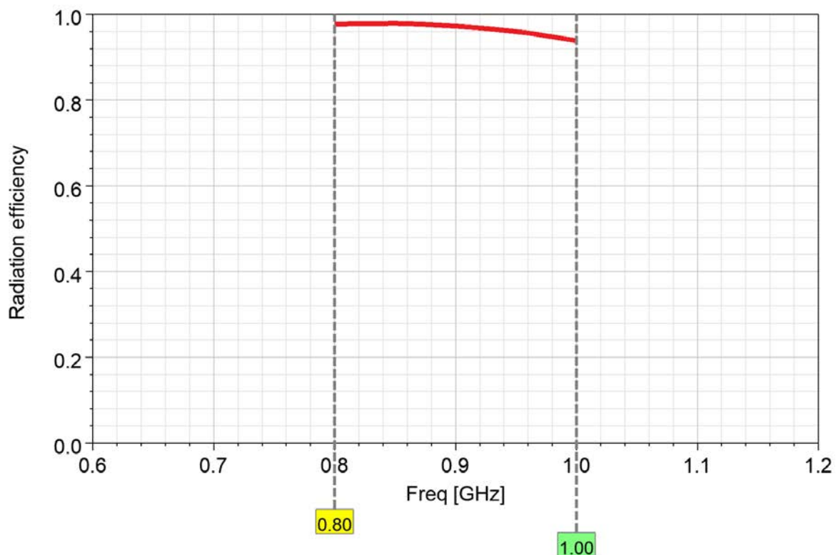
Radiation efficiency
