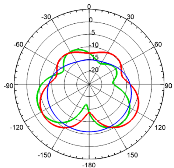
400 MHz
