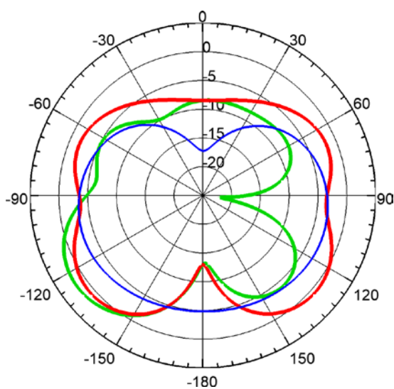
600 MHz
