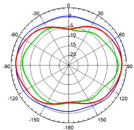
800 MHz
