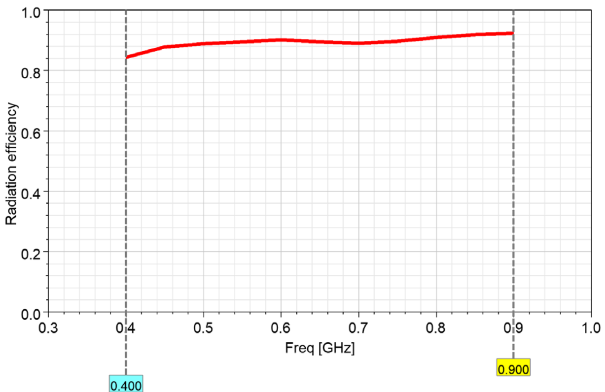
Radiation efficiency
